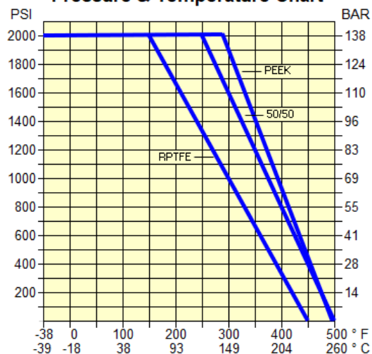
Pressure & Temperature Chart
