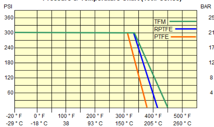
Pressure &amp; Temperature Chart (150# Series)
