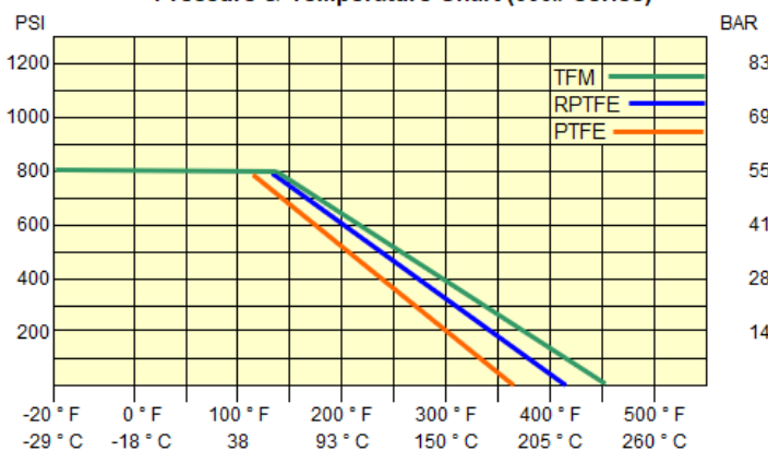
Pressure &amp; Temperature Chart (300# Series)
