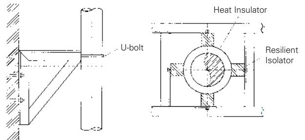
Sway brace ( ++ )
