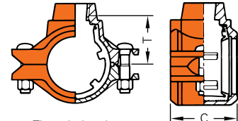
Threaded outlet
