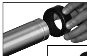
Fast-Fit™ Gasket: Easy installation with a single hand
