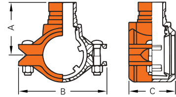
Grooved outlet
