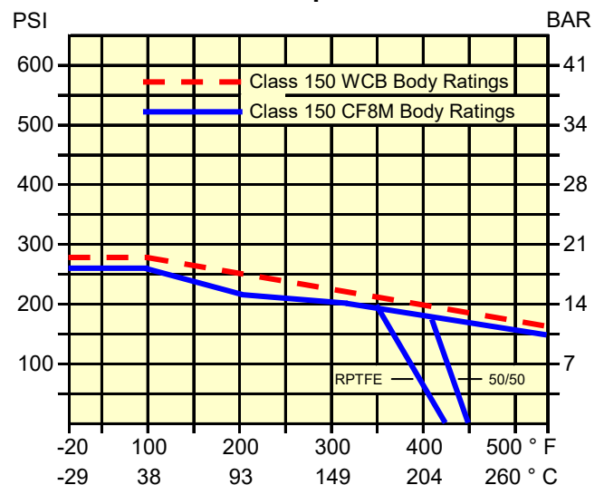
Pressure & Temperature Chart
